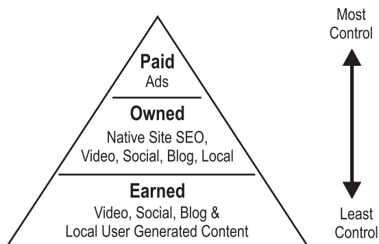
Fig. 1. SERP Categorization
