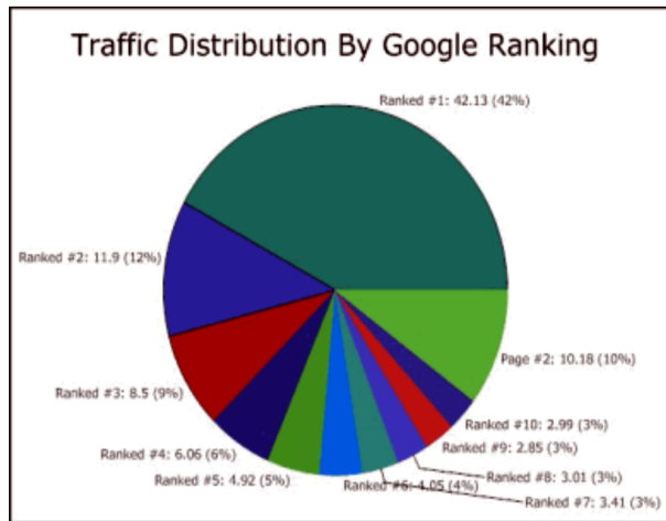
Fig. 2. Traffic distribution
