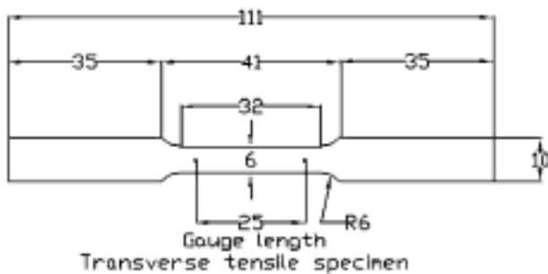
Fig. 4 Transverse Tensile Specimen
