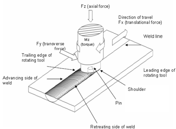
Fig. 1 Schematic of the FSW Process [3]
