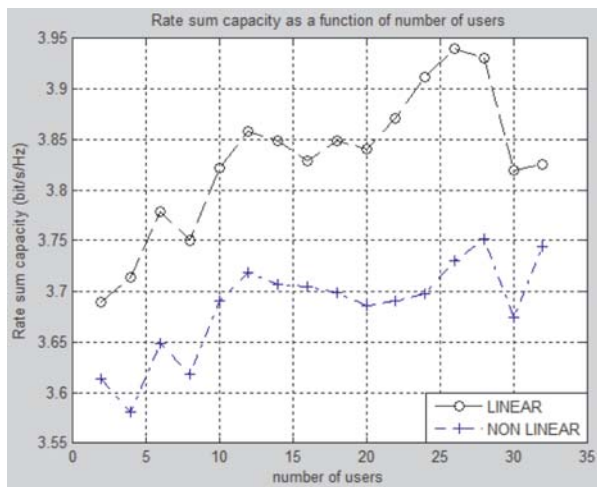
Fig. 2. Number of users verses Rate sum capacity in uplink OFDMA system
