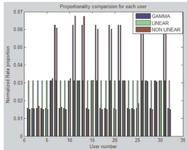
Fig. 4. User number verses normalized rate proportions in uplink OFDMA system
