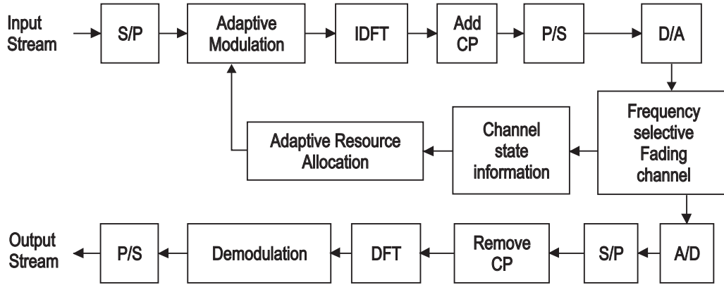
Fig. 1. Block Diagram of Uplink OFDMA system
