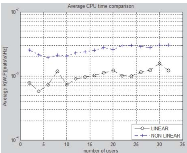
Fig. 3. Number of users verses Average Rate time in uplink OFDMA system
